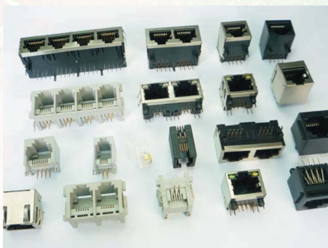
Telephone Jacks & RJ45 Jacks Series 电话插座及RJ45插座系列
