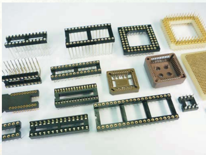
DUAL-IN-LINE Sockets & PGA Sockets Series IC 插座及 PGA 插座系列
