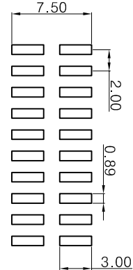
RECOMMENDED PCB LAYOUT COMPONENT SIDE VIEW
