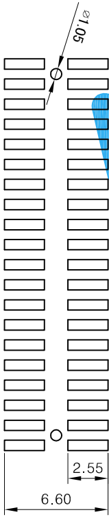
RECOMMENDED PCB LAYOUT COMPONENT SIDE VIEW
