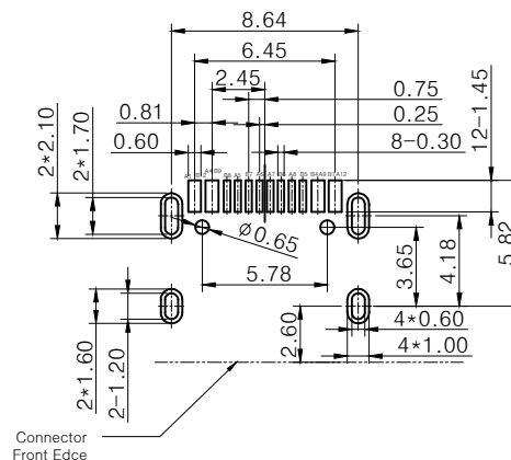
P.C.B. Layout Tolerance Unspecified±0.05mm
