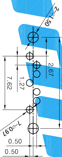
RECOMMENDED PCB LAYOUT COMPONENT SIDE VIEW
