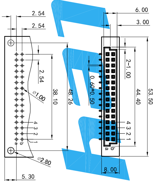
PCB LAYOUT(RECOMMENDED)
