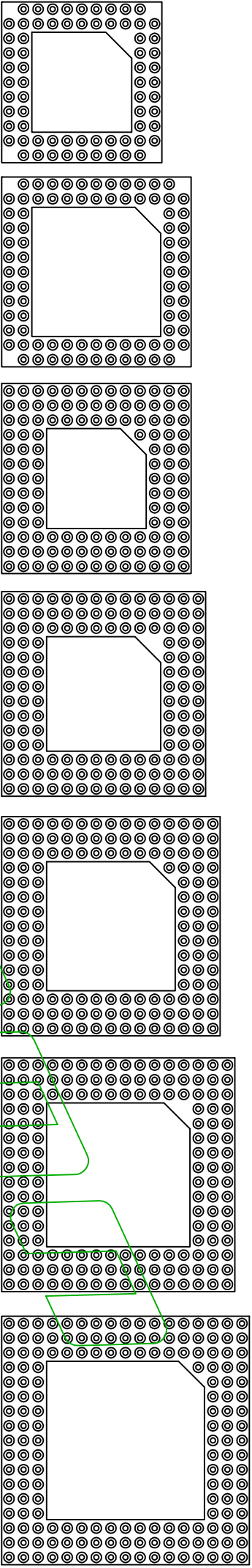
PGA basic body 11X11 PGA basic body 13X13 PGA basic body 13X13 PGA basic body 14X14 PGA basic body 15X15 PGA basic body 16X16 PGA basic body 17X17 Number of contacts: 68 Number of contacts: 84 Number of contacts: 121 Number of contacts: 132 Number of contacts: 145 Number of contacts: 156 Number of contacts: 169
