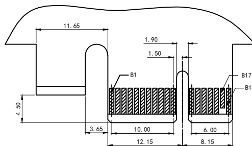
RECOMMENDED EDGE CARD PATTERN (PRIMARY SIDE)
