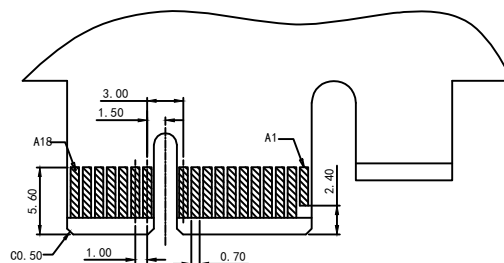
RECOMMENDED EDGE CARD PATTERN (SECONDARY SIDE)
